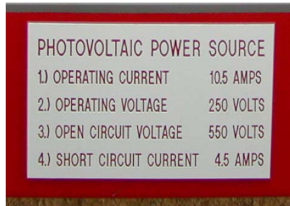
Figure 10 PV Power Source Sign
