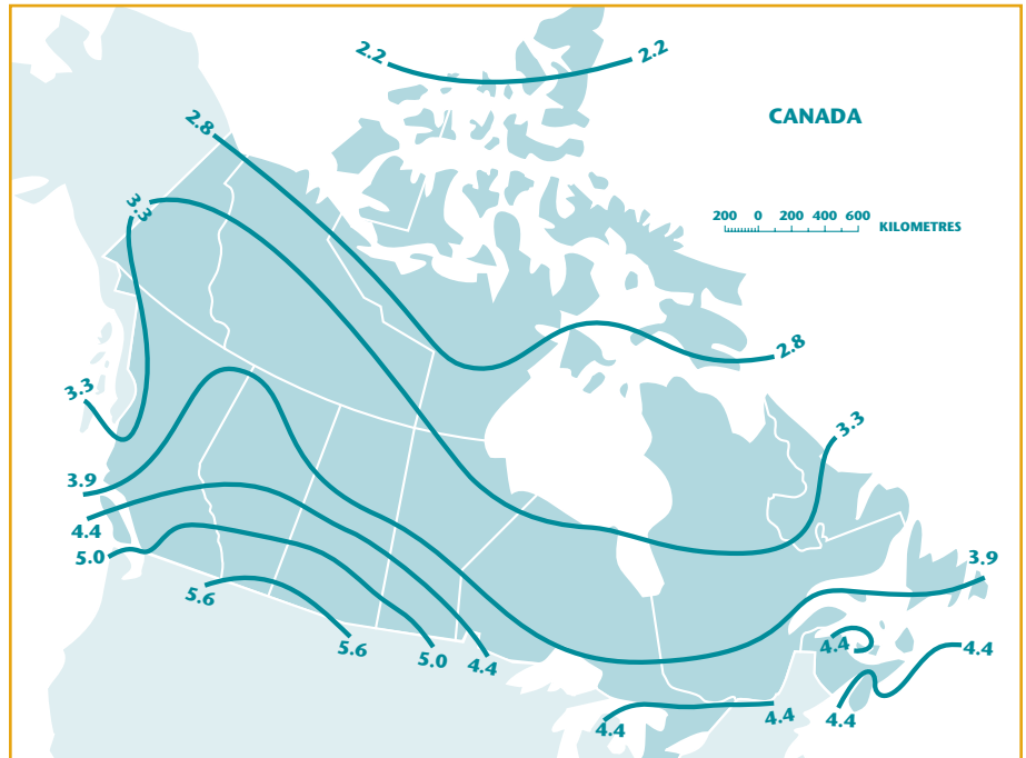
▲ Average daily number of peak sunlight hours in September (use for seasonal summer autonomous systems). Source: Environment Canada.
