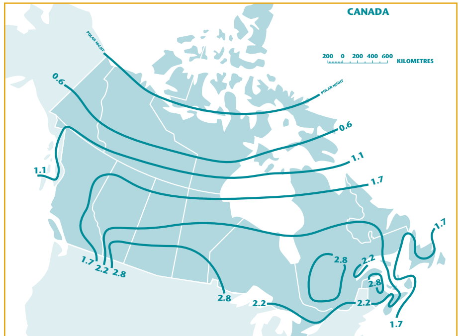
▲ Average daily number of peak sunlight hours in December (use for year-round-operated autonomous systems). Source: Environment Canada.
