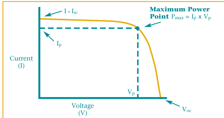
▲ Important points that characterize a PV module.
