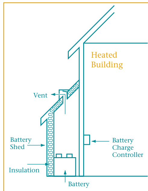
▲ Battery housed in a shed.
