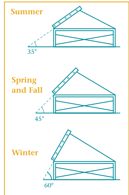
▲ Array orientations showing suggested tilt angles for summer, spring and fall and winter use in southern Canada.
