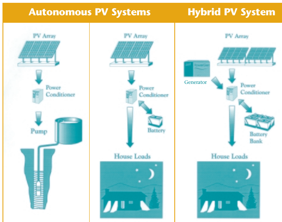
▲ Autonomous PV system without batteries.
