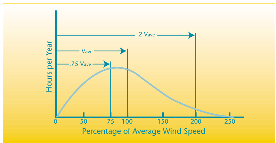
▲ Figure 3. Annual Average Wind Speed ( V_{ave} ) The high point of the curve is the speed at which the wind blows most often. Such a graph is called a Rayleigh wind speed distribution curve .
